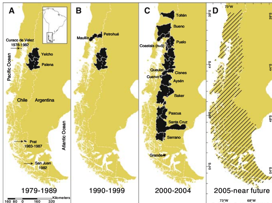
Fig. 1 Range expansion of Chinook salmon in South America. Locations and years of smolt releases for ocean ranching are shown with arrows in panel A. The black areas are basins (only labeled when first noted) where the species has been captured freeranging as (A, B) reported in empirical studies, and (C) based on empirical studies, angler interview surveys, media
